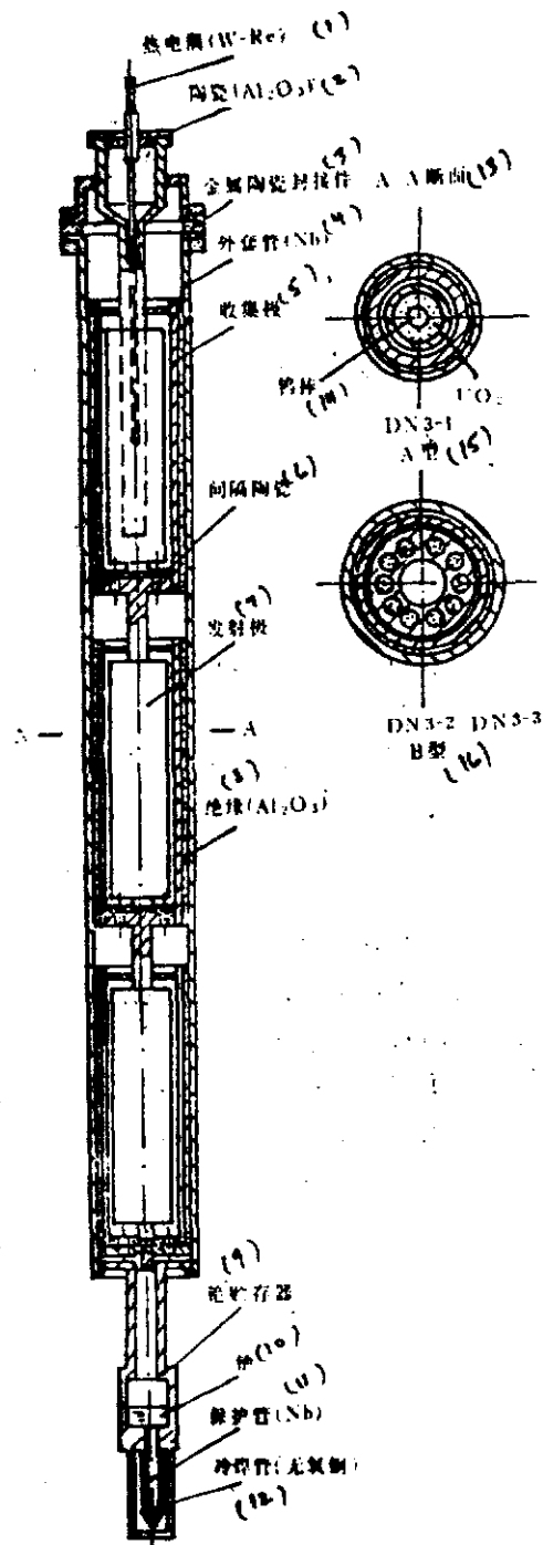
Fig. 1. Thermionic converter in-pile experimental installation. Key is at right of figure.
